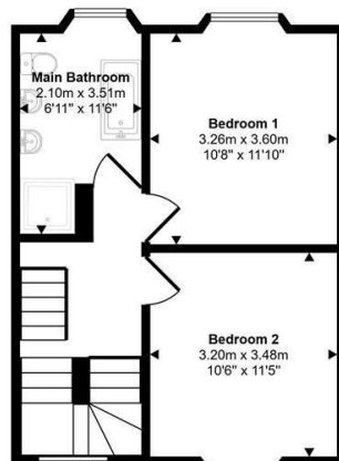
First Floor Approx 41 sq m / 437 sq ft
